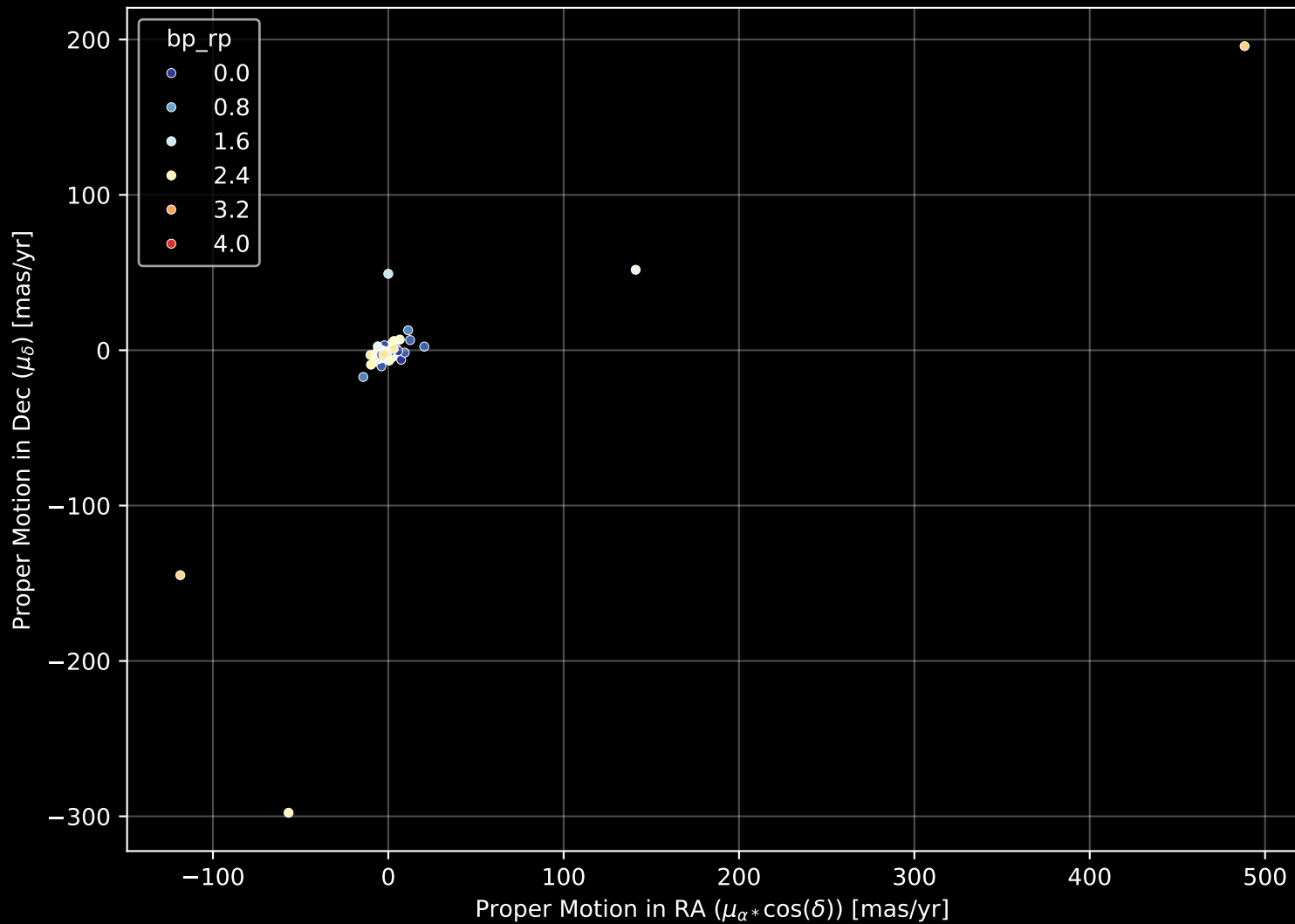
APOGEE DR17 Field: [098+04] Proper Motion Diagram (n= 188)
