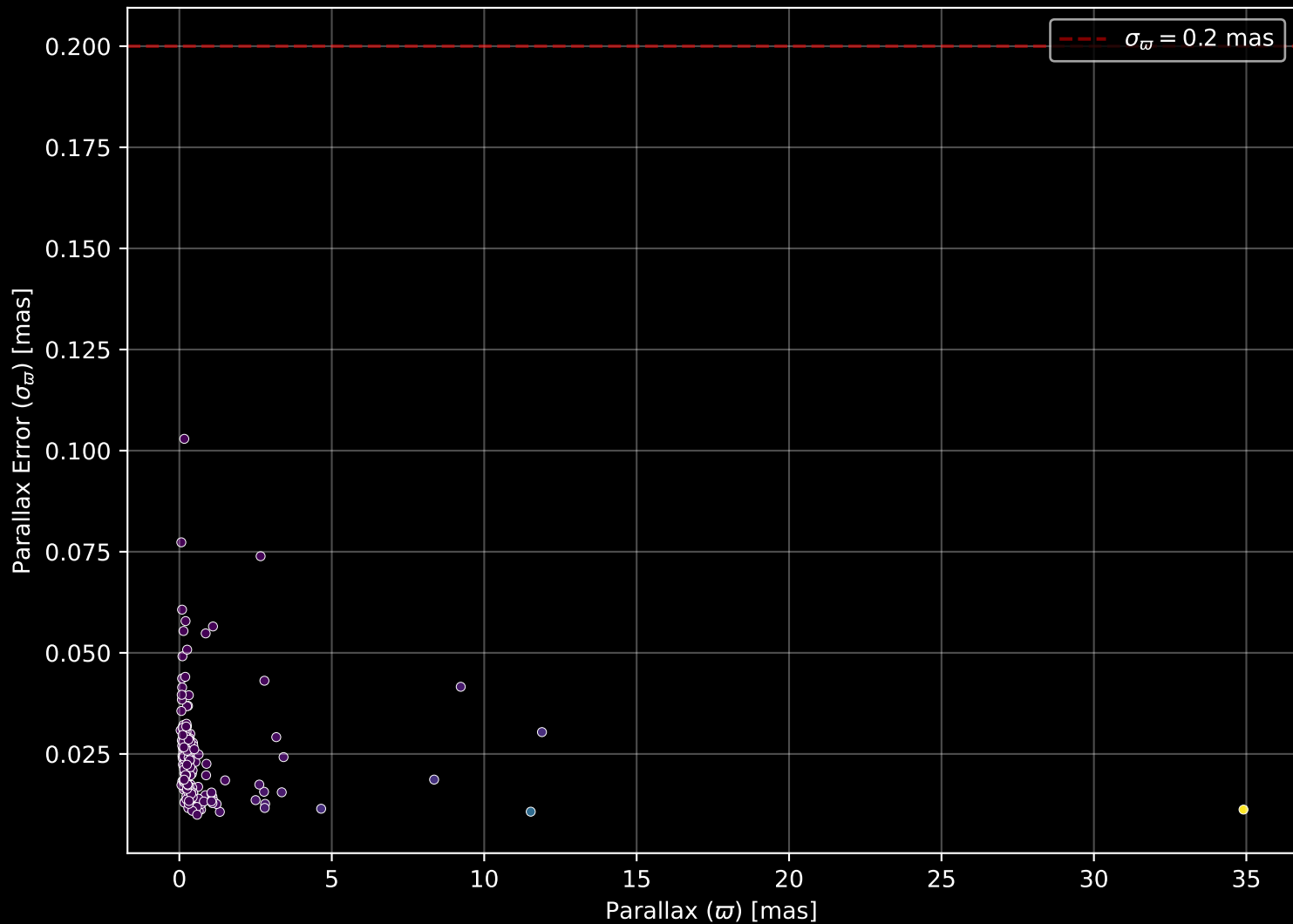
APOGEE DR17 Field: [098+04] Parallax Quality (n= 188)
