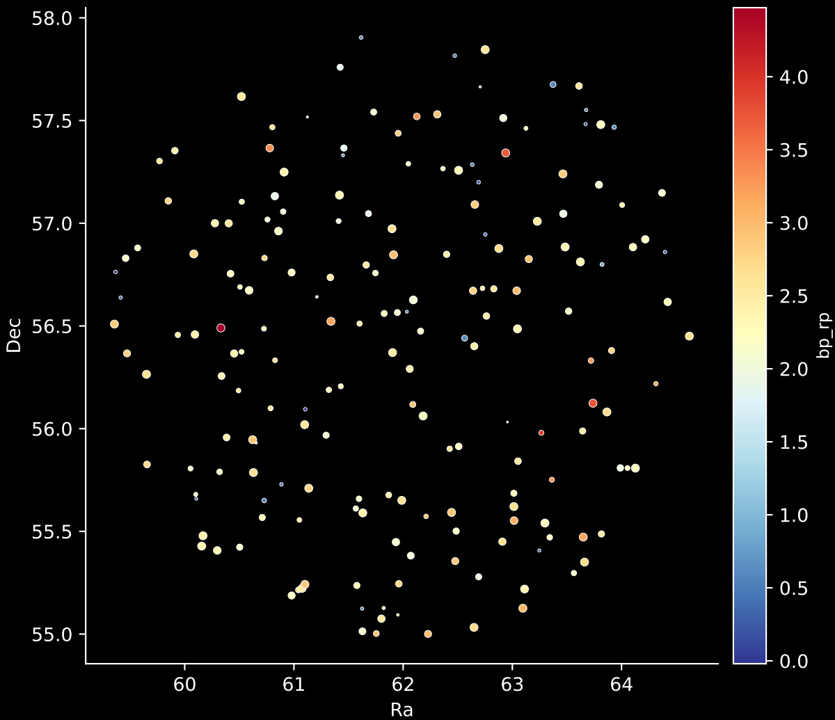
APOGEE DR17 Field: [098+04] Stars: 188
