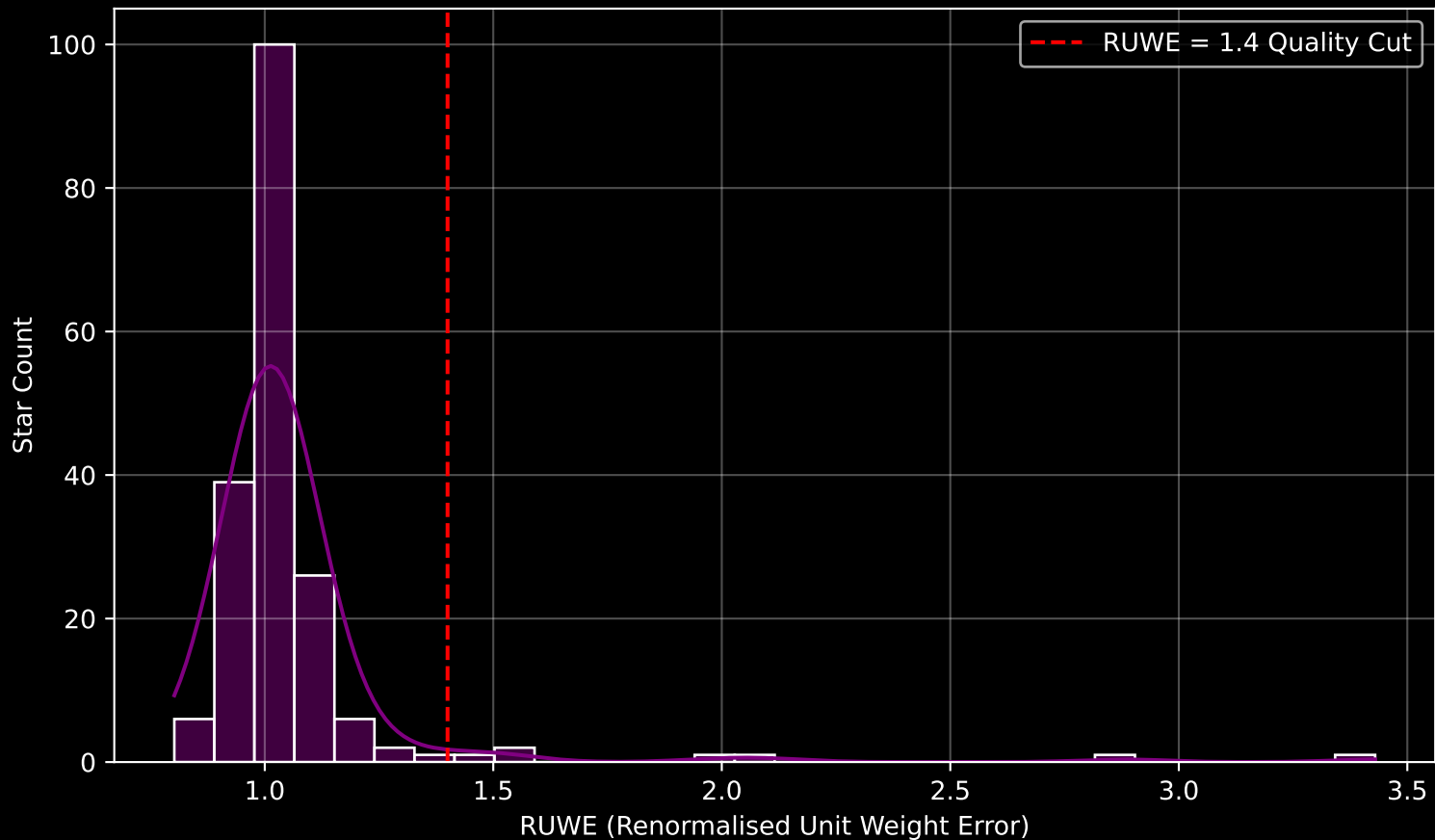
GAPOGEE DR17 Field [098+04] RUWE Distribution (n= 187)
