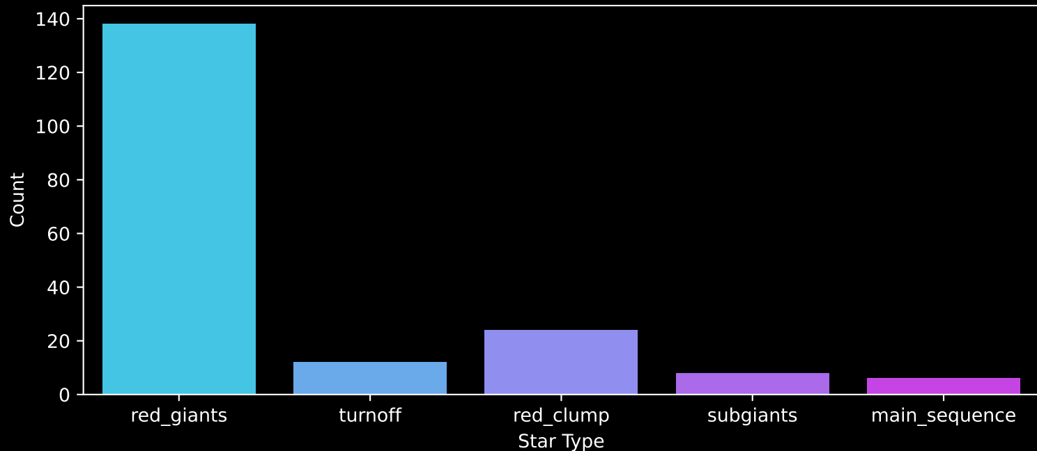
APOGEE DR17 Field: [098+04] Count plot of Star Type
