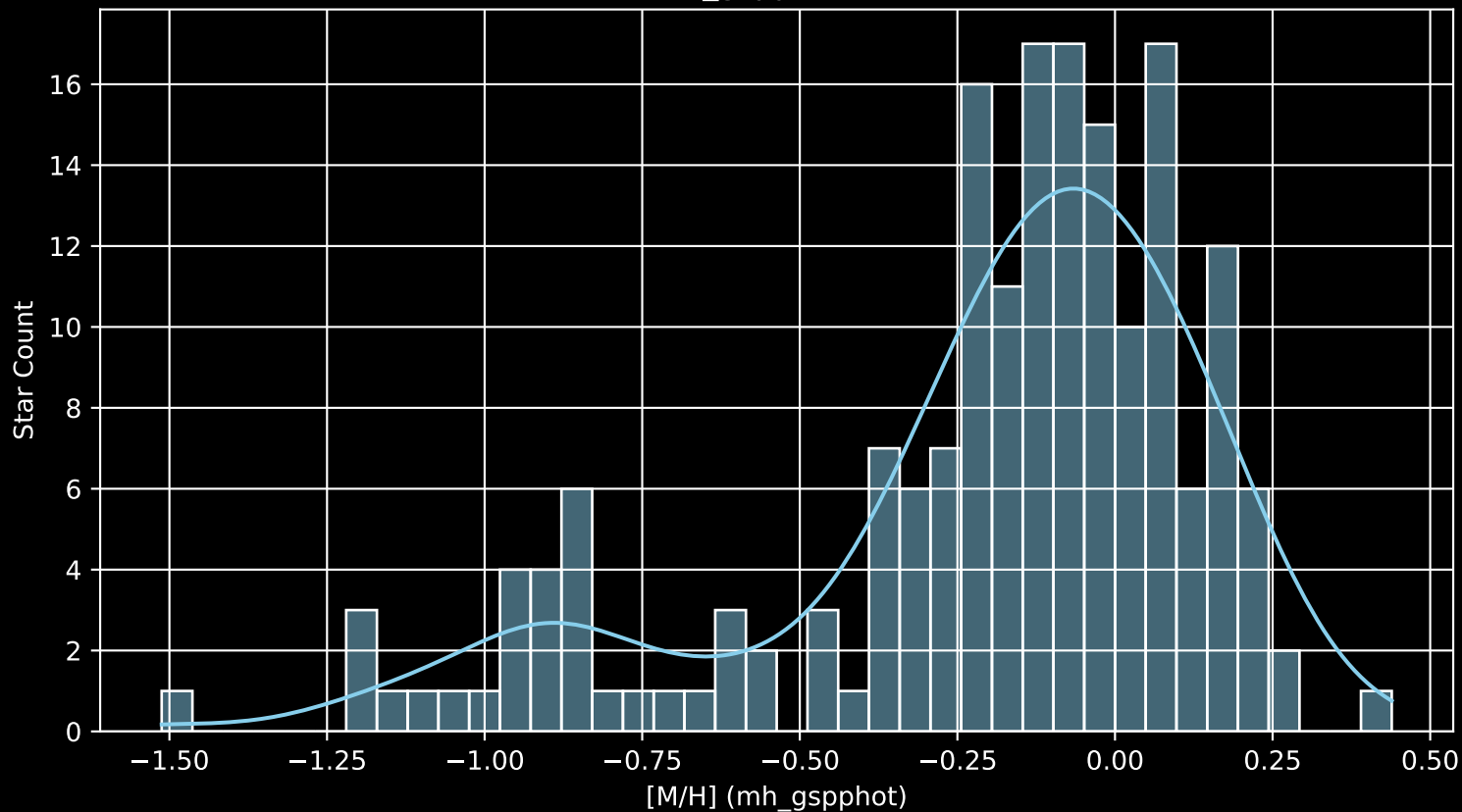
APOGEE DR17 Field: [098+04 [M/H] (mh_gspphot) (n= 185)
