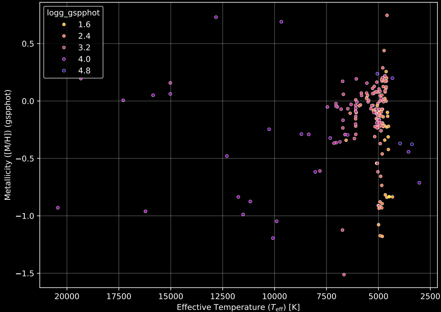
APOGEE DR17 Field: [098+04] Stellar Population Parameters (n= 188)
